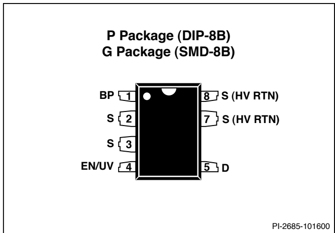
Figure 3. Pin Configuration.
