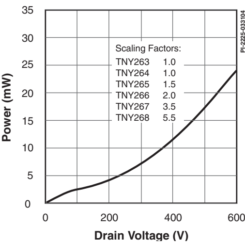
Figure 29. Drain Capacitance Power.
