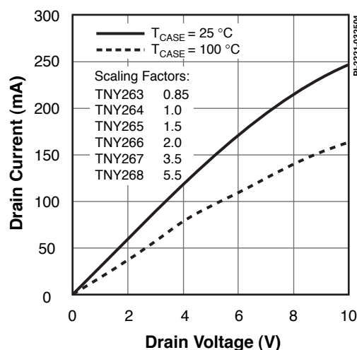
Figure 27. Output Characteristic.
