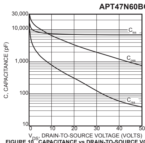
FIGURE 10, CAPACITANCE vs DRAIN-TO-SOURCE VOLTAGE
